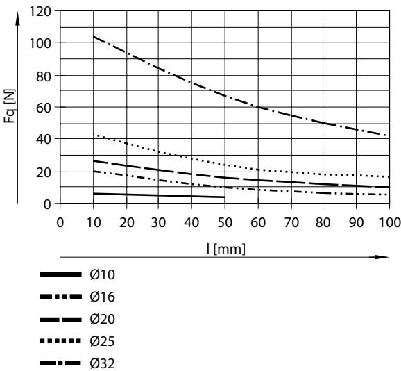
Permissible transverse load F as a function of stroke L - Single-sided Piston rod - Plain-bearing guide
