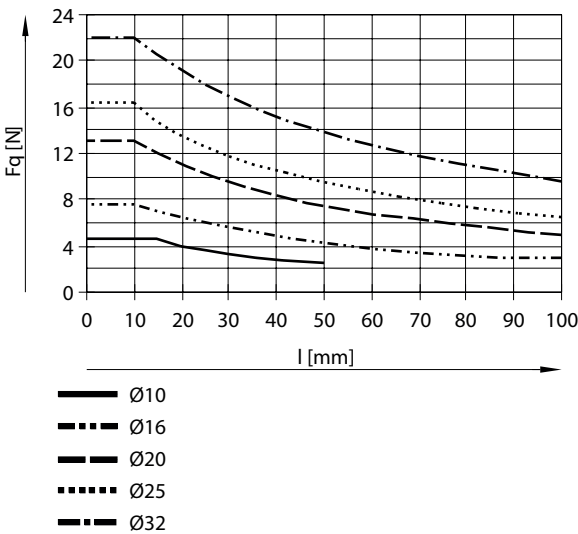
Permissible transverse load F as a function of stroke L - Single-sided piston rod - Recirculating ball guide
